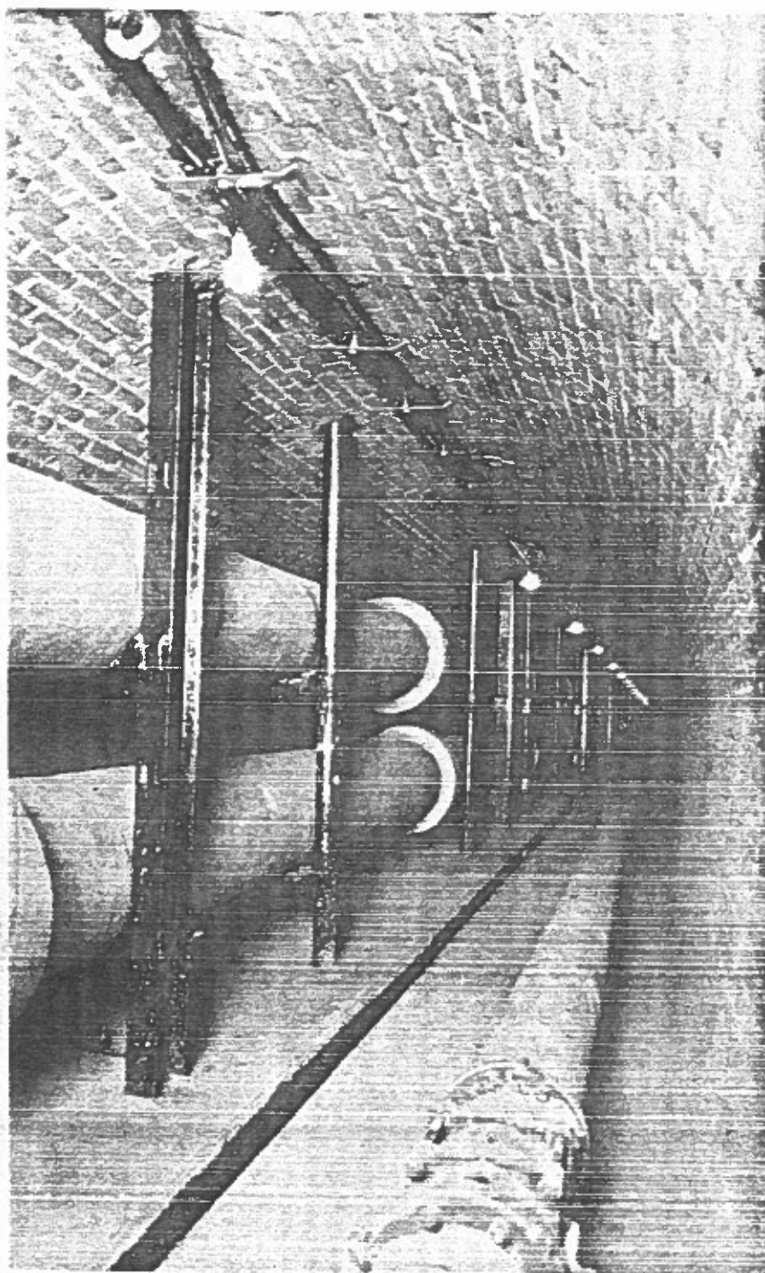
Fig. 20—Beacon-Woodward Tunnel
