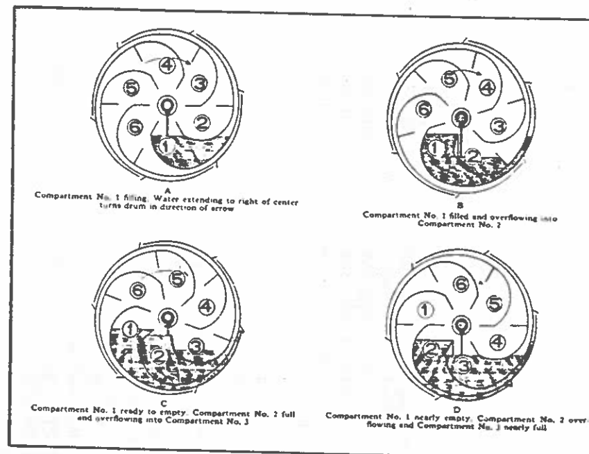
Fig. 22—Condensation Meter, Cycle of Operation
