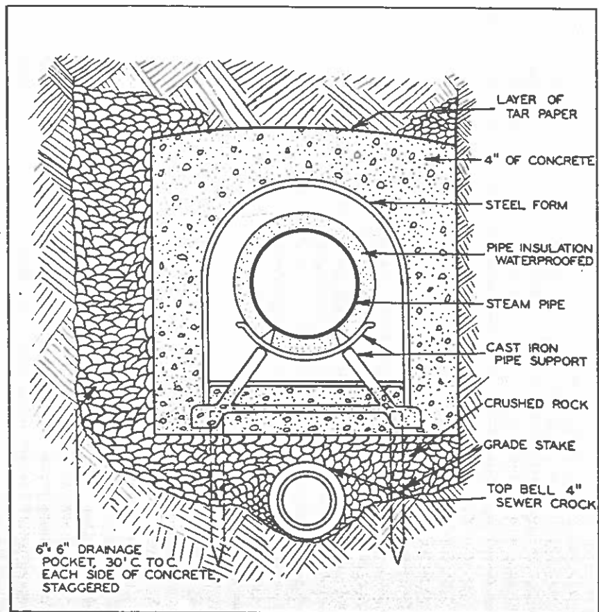
Fig. 19—Concrete Construction for Underground Steam Lines
