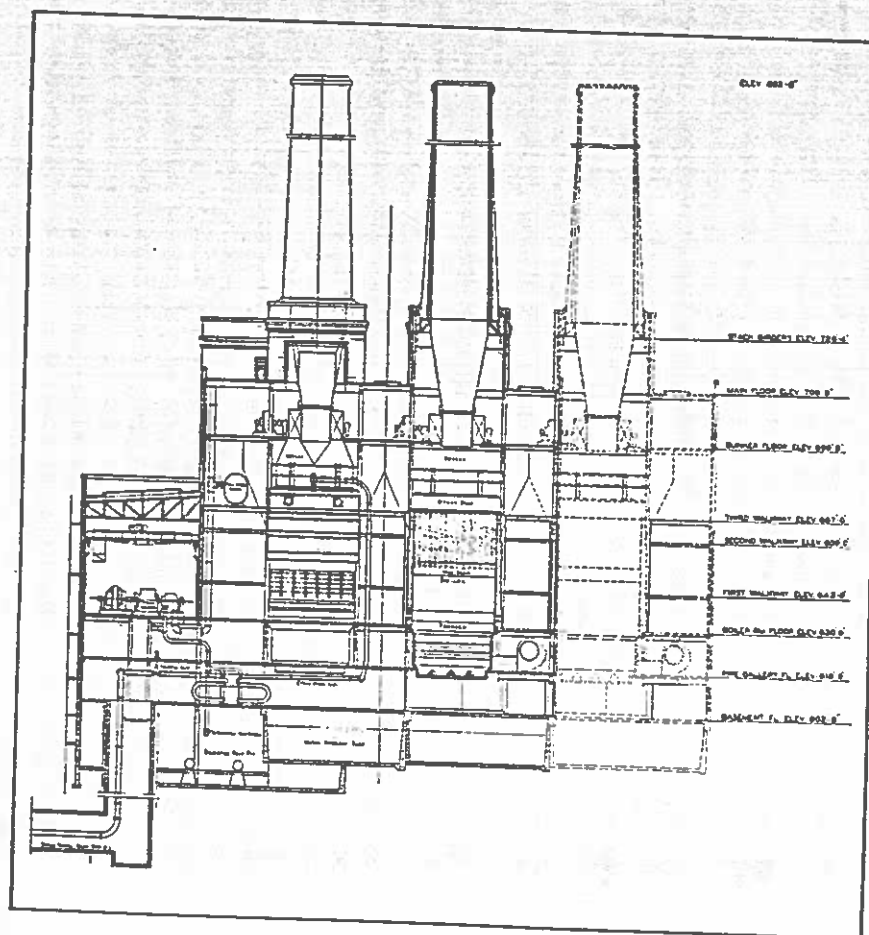
Fig. 12—Longitudinal Section, Beacon Street Heating Plant
