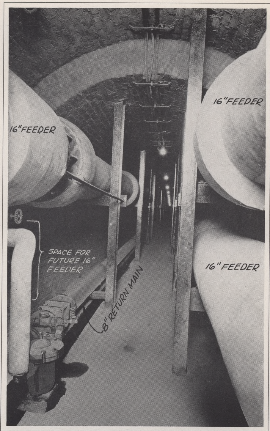
Fig. 21—Beacon-Woodward Tunnel
