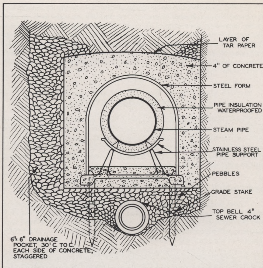
Fig. 20—Concrete Construction for Underground Steam Lines
