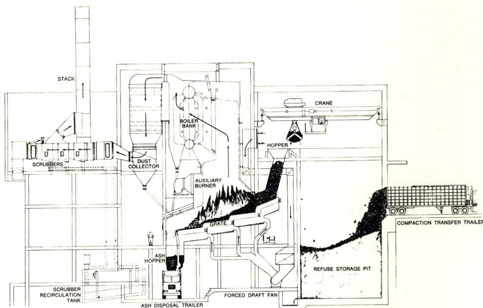
FIG. 2—Schematic diagram of one of the large incinerator-boilers. Solid waste will be delivered by truck (right) and dumped into a large refuse storage pit. An overhead crane will pick up the refuse in one-ton bites and deliver it to the charging hopper. Moving grates will carry the refuse through the combustion chamber, where heat rising from the burning
