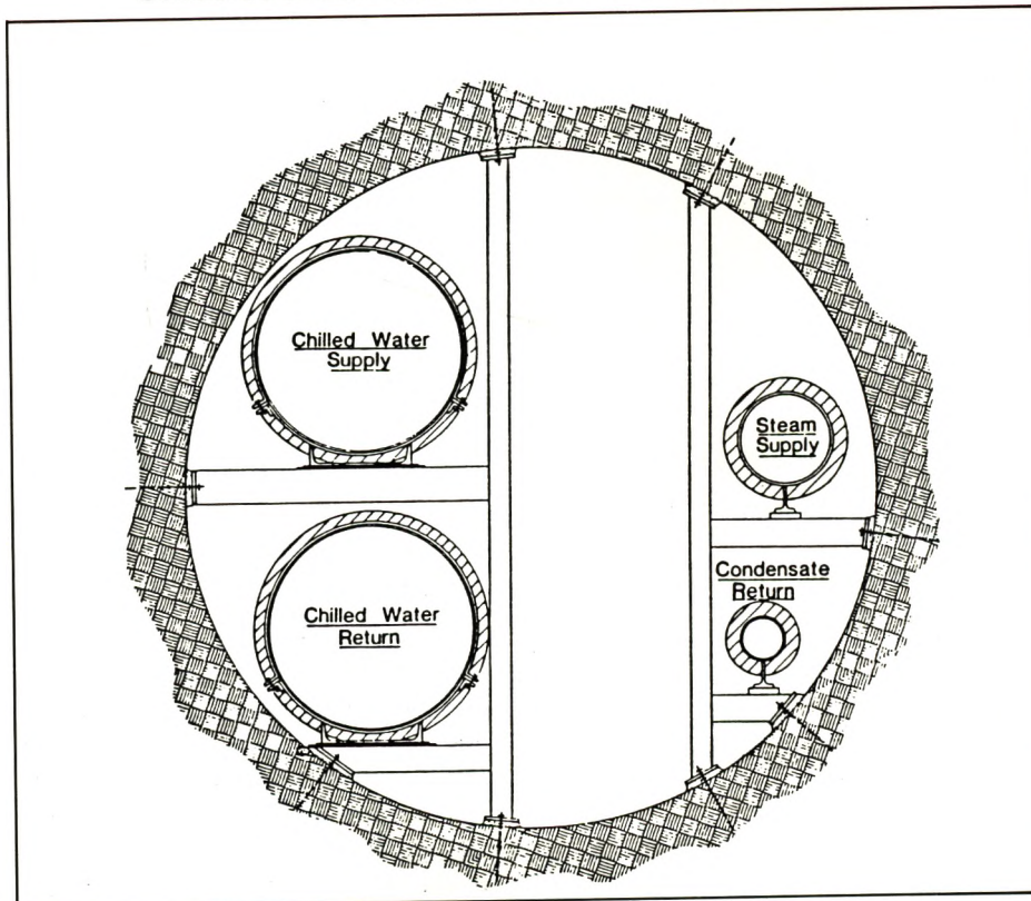
FIGURE 4 Cross section of Nashville's distribution tunnel
