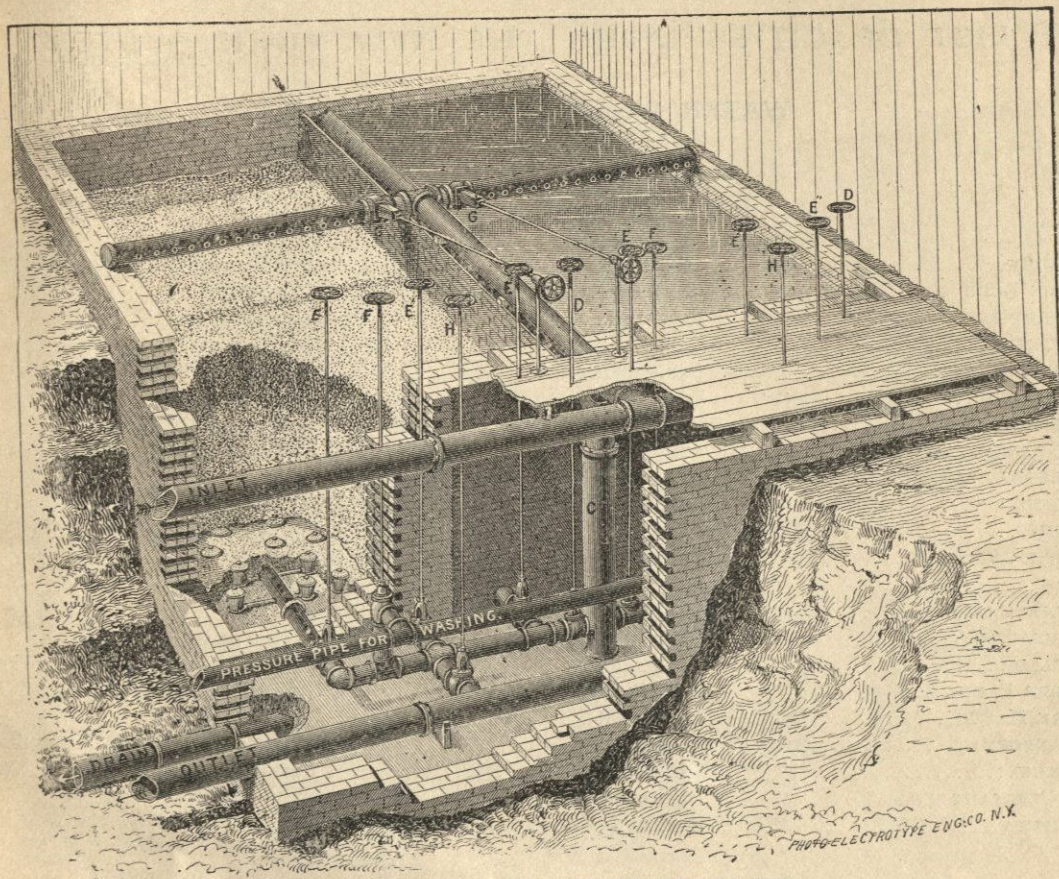
BRICK SECTIONAL WASHING GRAVITY FILTER.
