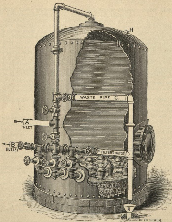
Cut of Filters from 24 inches Diameter up to 10 feet Diameter.
