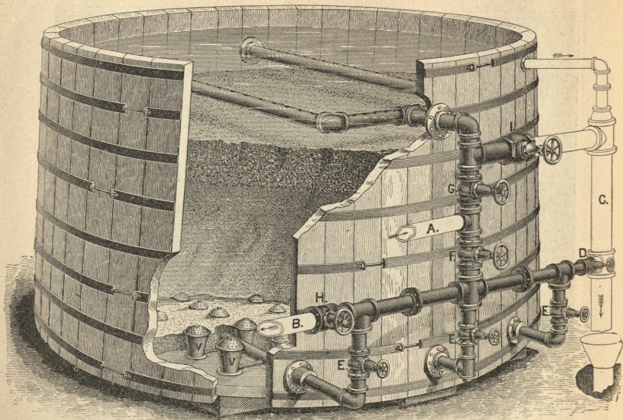
WOODEN SECTIONAL WASHING GRAVITY FILTER.
